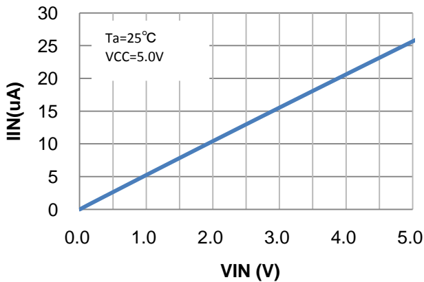
Figure 6. Input current vs. Input voltage
