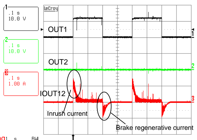
Figure 18. Driving waveform of DC motor
