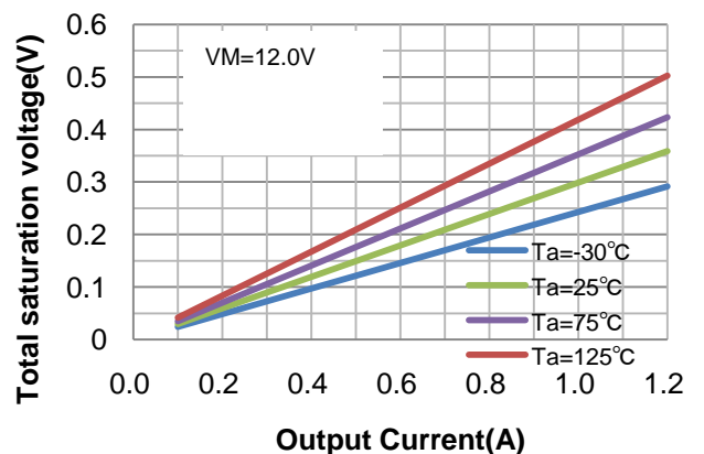
Figure 9. Saturation voltage vs. Output current
