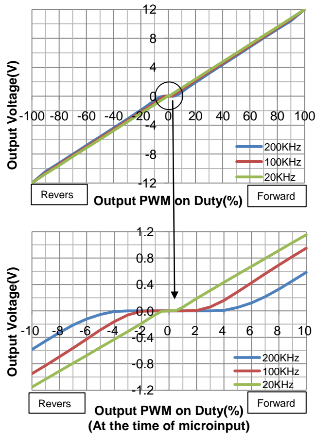
Figure 20. Input and Output Characteristics of H-Bridge
