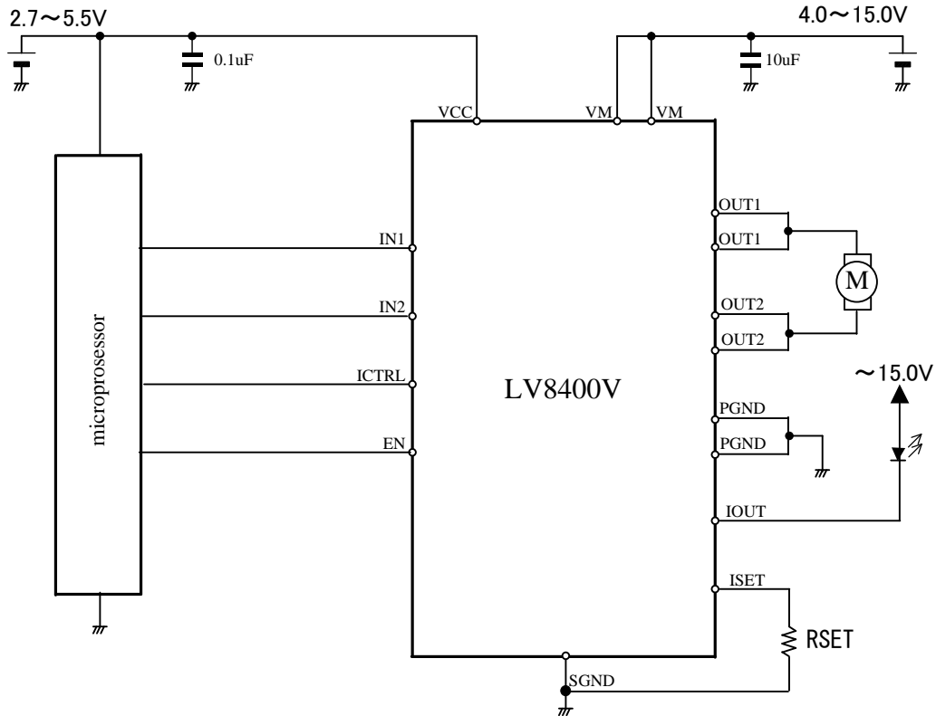
Figure 17. Sample Application Circuit
