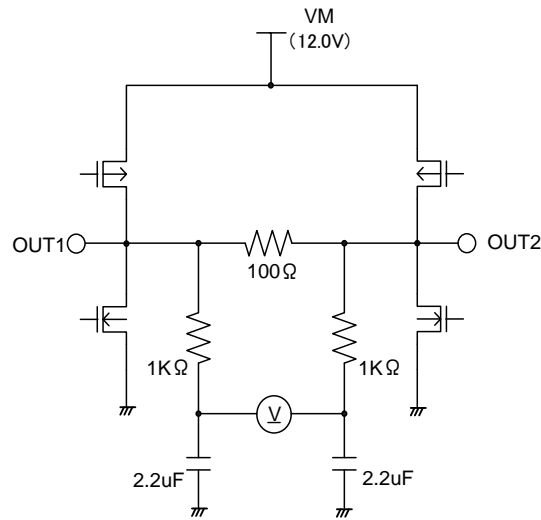
Figure 19.Measurement connection diagram
