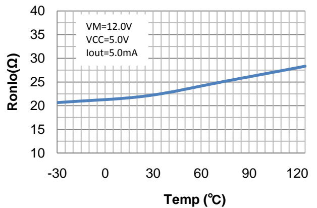
Figure 13. IOOUT on-resistance vs. Temperature
