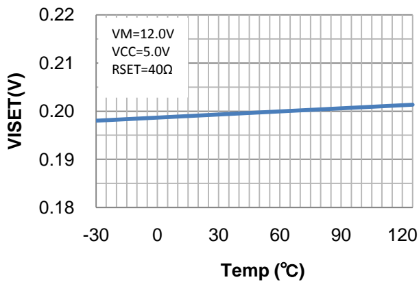
Figure 12. VISET voltage vs. Temperature
