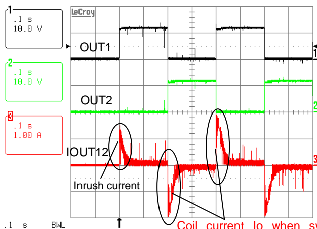
Coil current I_o when switching from forward to reverse
