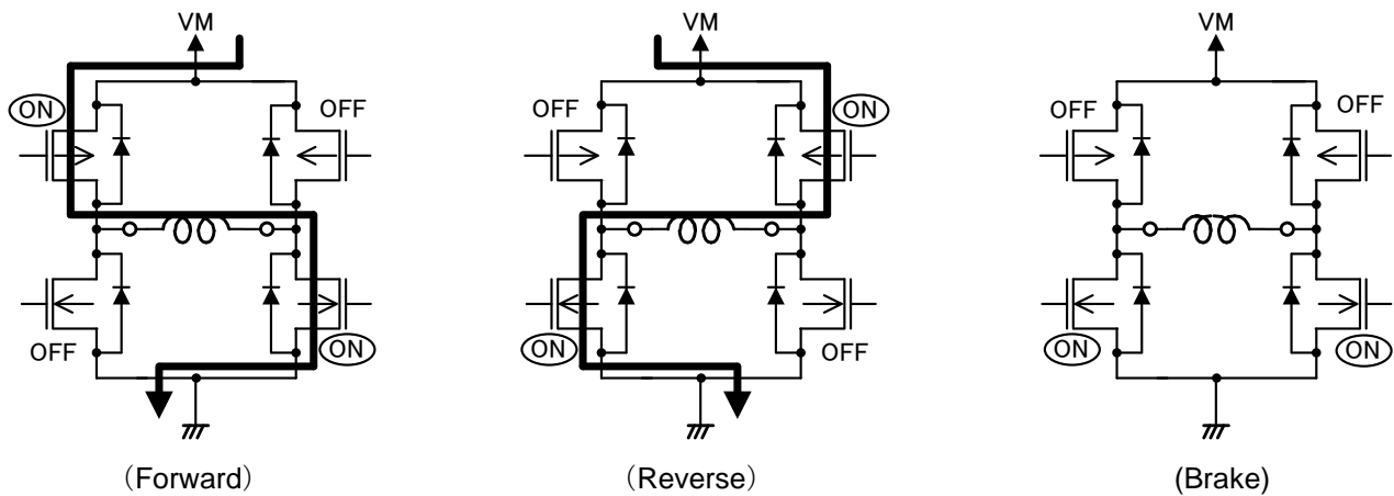
Figure 16. Output stage transistor function
