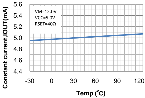
Figure 10. Constant current, IOOUT vs. Temperature
