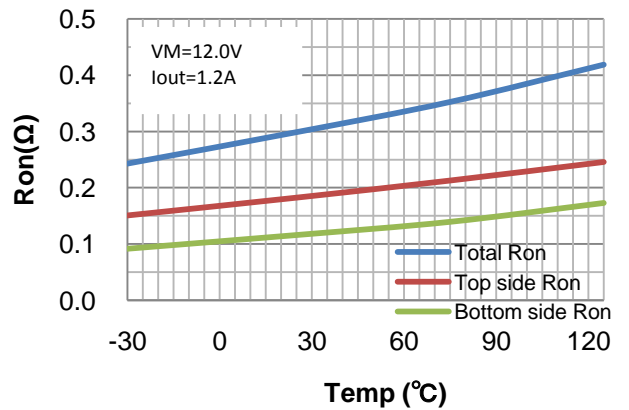
Figure 7. Output on-resistance vs. Temperature
