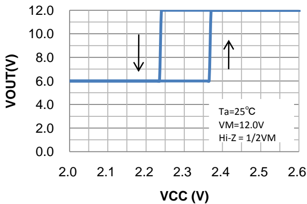
Figure 14. VCC low voltage reset characteristic
