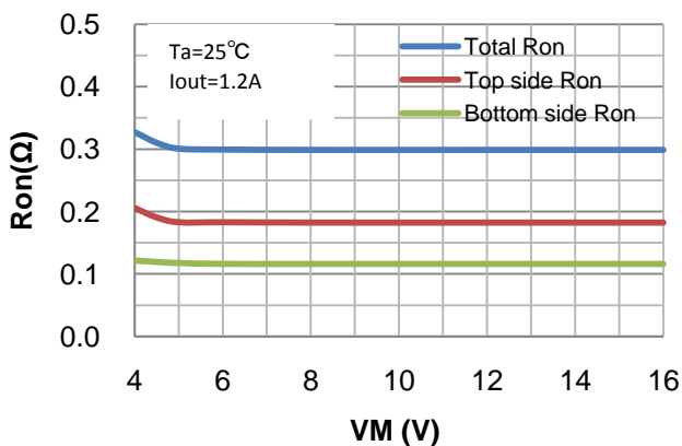
Figure 8. Output on-resistance vs. VM supply voltage
