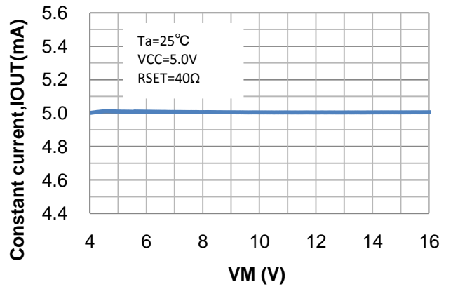
Figure 11. Constant current, IOOUT vs. VM supply voltage
