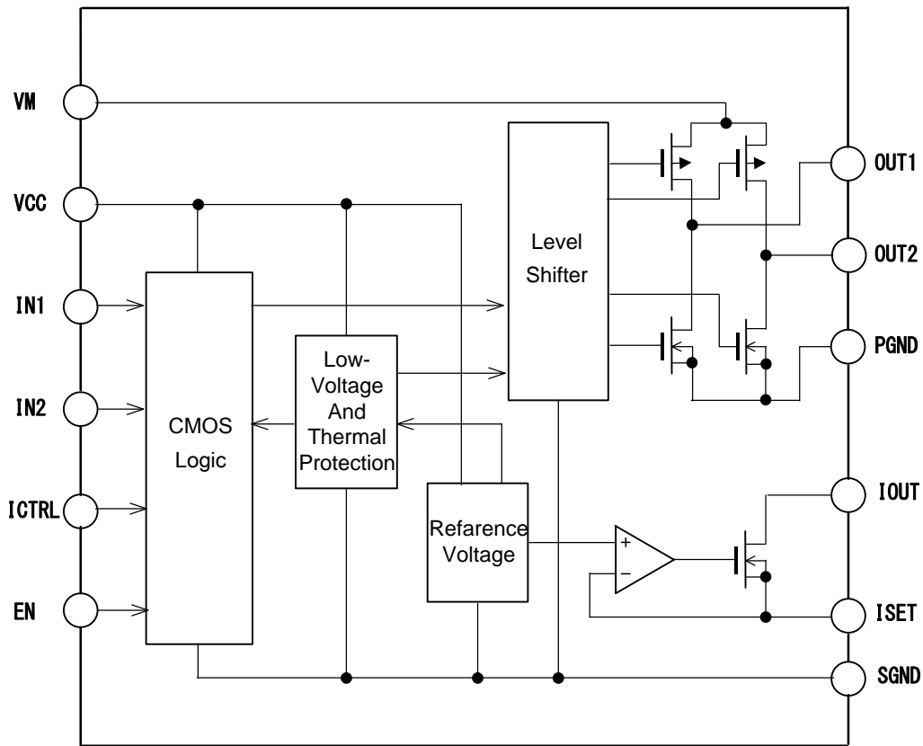
Figure 1. Block Diagram
