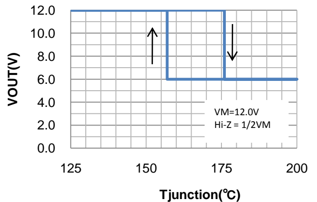
Figure 15. Thermal shutdown characteristic
